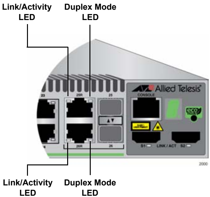
Figure 14. 10/100/1000Base-T Port LEDs
