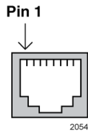
Figure 45. RJ-45 Socket Pin Layout (Front View)
