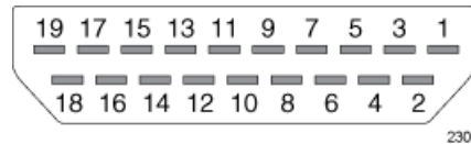
Figure 46. Stacking Port Pin Layout (Front View)
