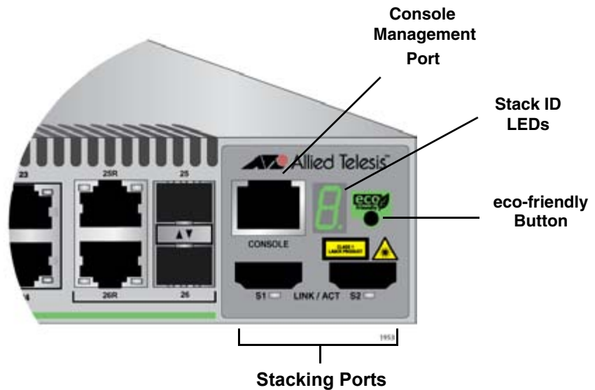
Figure 10. 8100S Series Management Panel
